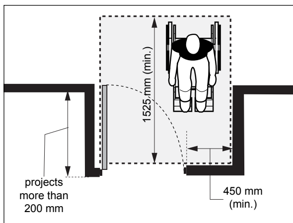
Figure 43a: Pull Side Approach at Recessed Side-Hinged Door - Plan View
