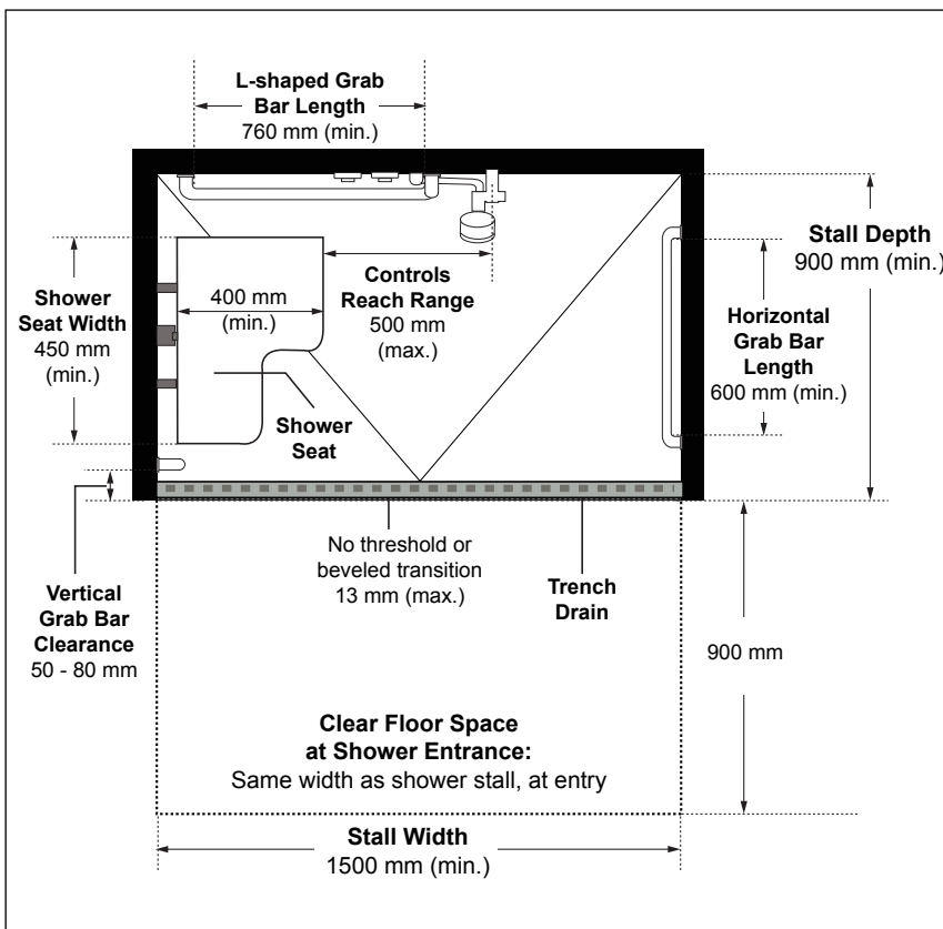
Figure 62: Shower Design and Layout - Plan View
