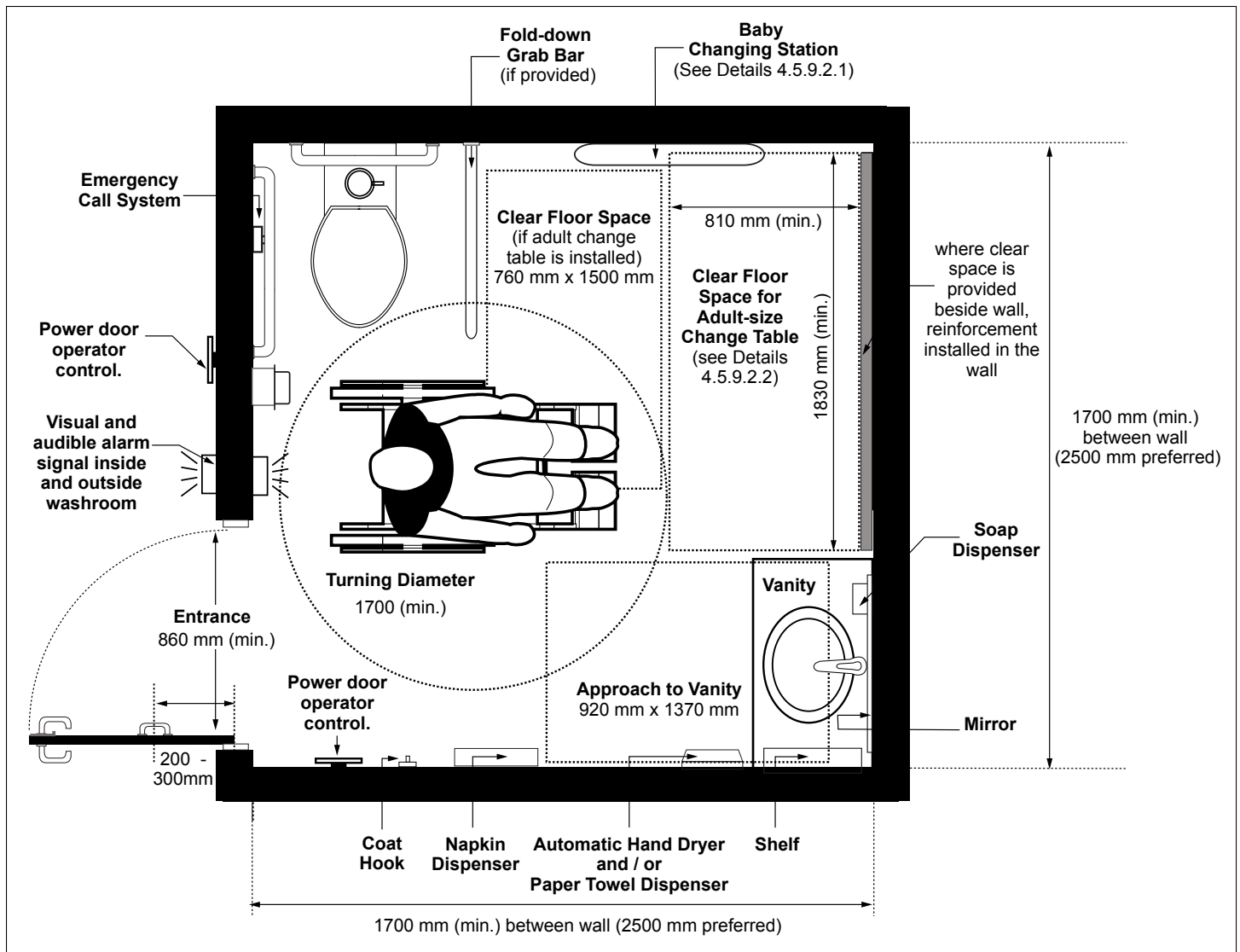
Figure 52: Universal Washrooms
