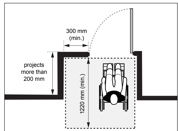
Figure 43b: Push Side Approach at Recessed Side-Hinged Door - Plan View
