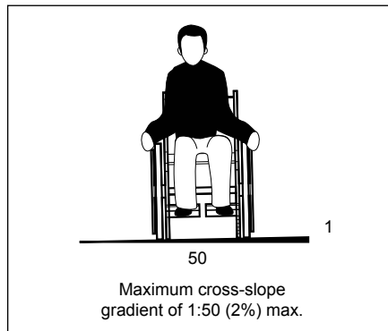
Figure 50: Cross-Slope
