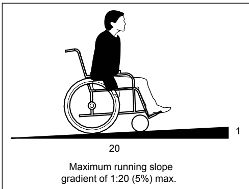
Figure 49: Running Slope
