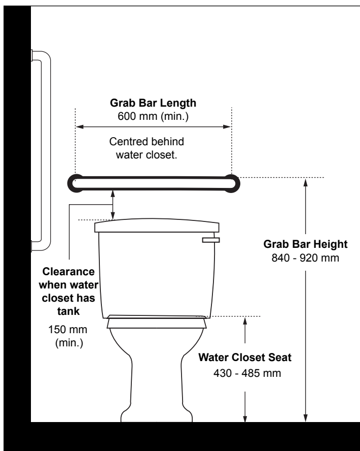
Figure 55: Horizontal Grab Bar (Water Closet with Water Tank)
