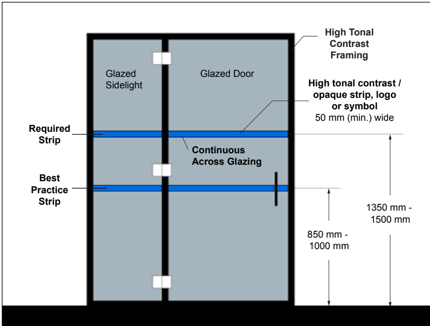
Figure 45: Glazed Doors - Elevation View
