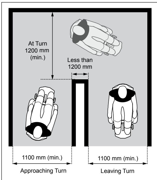
Figure 48a: 180 Degree Turn (Typical)
